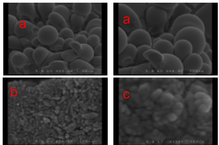
Fig. 3 SEM images of CuPcTs nanoparticles
