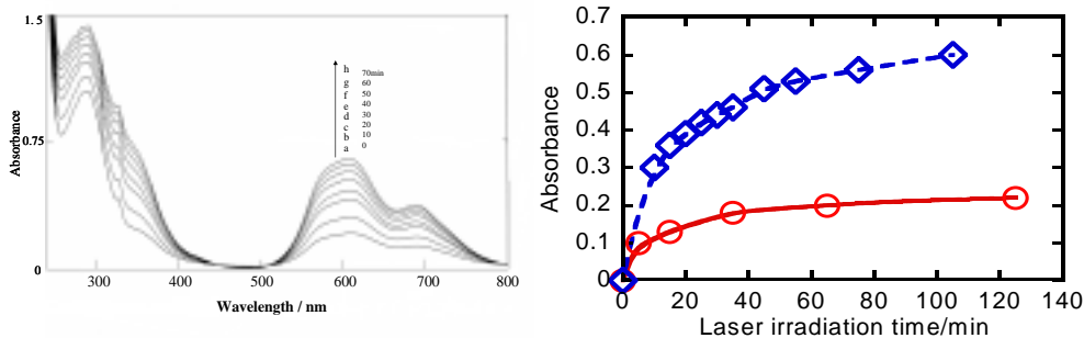
Fig. 2 (A) Laser-irradiation time dependence of absorption spectra and (B) laser-irradiation time dependence of absorbance of CuTsPc particles in methanol.
