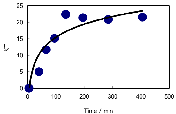
Fig. 4 Laser irradiation time dependence of IRAS band for CuPcTs particles.
